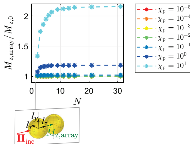
Figure 9. Maximum magnetization in a line of spherical para-/ferromagnetic particles normalized to the magnetization of a single particle without in absence of the other particles.
